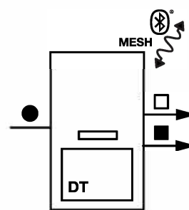
S-OC-024-D00W DUAL-TECH WALL OCC SENSOR PIR + HIGH FREQUENCY DOPPLER SURFACE WALL OR CEILING MOUNT 4.4"x2.6"x1.8" (112x66x46MM) POWER SUPPLY 22-26 VDC/DC INSTALL WITHIN 30' OF CLOSEST DEVICE
