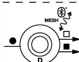
S-DL-C12-DTWH DAYLIGHT + OCC PIR SENSOR 3.66" (93MM) DIAMETER RECESS CEILING MOUNT / 10FT (3M) INPUT 12-24VDC | NEEDS AC/DC TRANSFORMER OR AUXILIARY DC OUTPUT OF BUBBLYNET CONTROLLER INSTALL WITHIN 30' OF CLOSEST DEVICE
