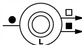
S-OP-012-D0LB LOW BAY PHOTOCELL + PIR OCC SENSOR 3.66" (93MM) DIAMETER SURFACE CEILING MOUNT / UP TO 30' (9.1M) INPUT 12-24VDC | NEEDS AC/DC TRANSFORMER OR AUXILIARY DC OUTPUT OF BUBBLYNET CONTROLLER INSTALL WITHIN 30' OF CLOSEST DEVICE
