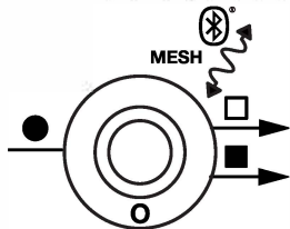
S-OP-C12-DTWH OCC + PHOTOCELL PIR SENSOR 2.68" (68MM) DIAMETER RECESS CEILING MOUNT / 10FT (3M) INPUT 12-24VDC | NEEDS AC/DC TRANSFORMER OR AUXILIARY DC OUTPUT OF BUBBLYNET CONTROLLER INSTALL WITHIN 30' OF CLOSEST DEVICE
