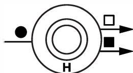
S-OP-012-D0HB HIGH BAY PHOTOCELL + PIR OCC SENSOR 3.66" (93MM) DIAMETER SURFACE CEILING MOUNT / UP TO 40' (12.2M) INPUT 12-24VDC | NEEDS AC/DC TRANSFORMER OR AUXILIARY DC OUTPUT OF BUBBLYNET CONTROLLER INSTALL WITHIN 30' OF CLOSEST DEVICE
