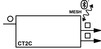
CT2C C-T2C-24-DS00 DUAL CH, 0-10V TUNABLE WHITE CONTROLLER 3.25"x1.5"x0.875" (82.5x38x22mm) INPUT 12-24 VDC | OUTPUT 0-10VDCx2CH INSTALL WITHIN 60' OF CLOSEST DEVICE
