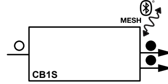
CB1S C-B1S-24-DS00 BEAM SHAPER CONTROLLER 3.25"x1.7"x1.36" (90x43.2x34.5mm) INPUT 24 VDC | OUTPUT 4 PIN ZOOM LENS INSTALL WITHIN 60' OF CLOSEST DEVICE
