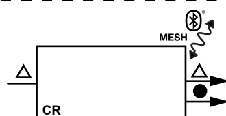
CR C-R00-11-DL00 REVERSE PHASE CONTROLLER 5.25"x1.5"x1.25" (134x38x29mm) LINE INPUT 100-277VAC 200W MAX | AUXILIARY +24VC OUTPUT 100mA INSTALL WITHIN 60' OF CLOSEST DEVICE
