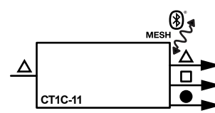
C-T1C-11 C-T1C-11-DL00 SINGLE CH 0-10V CONTROLLER WITH RELAY 5.25"x1.5"x1.125" (134x38x29mm) AC INPUT 110-277VAC OUTPUT RELAY 110-277VAC | 10 AMPS MAX 0-10V DIMMING 100mA MAX INSTALL WITHIN 60' OF CLOSEST DEVICE
