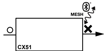
CX51 C-X51-24-DS00 DMX CONTROLLER 2.2" x 1.2" x 0.7" (72.6 x 30.0 x 18.0 mm) INPUT 12-24 VDC | OUTPUT 12-24 VDC INSTALL WITHIN 60' OF CLOSEST DEVICE
