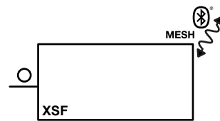
XSF X-SF-024-DS00 SUPERFRIEND CONTACT CONTROLLER 3.25"x1.5"x0.25" (82.5x38x6.35mm) INPUT 12-24 VDC | OUTPUT 0-10VDC INSTALL WITHIN 60' OF CLOSEST DEVICE
