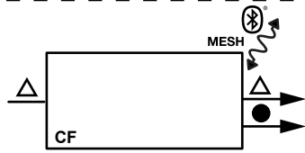
CF C-F00-11-DL00 FORWARD PHASE DIMMING CONTROLLER 5.25"x1.5"x1.25" (134x38x29mm) LINE INPUT 100-277VAC 200W MAX | AUXILIARY +24VC OUTPUT 100mA INSTALL WITHIN 60' OF CLOSEST DEVICE
